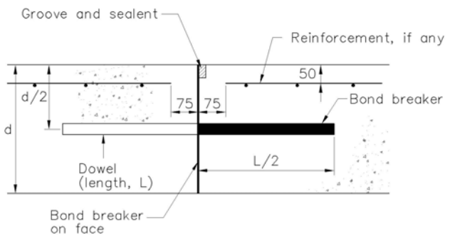
Figure 10B Dowelled butt joint
